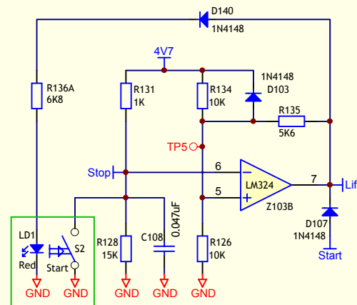
Electronic Start Circuit
