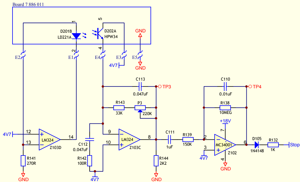
Electronic Start Circuit
