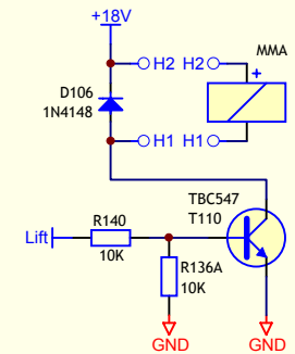
Lift Circuit
