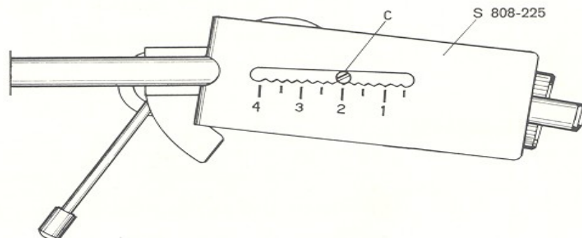
Fig. 9. Positioning the stylus force calibration plate.
