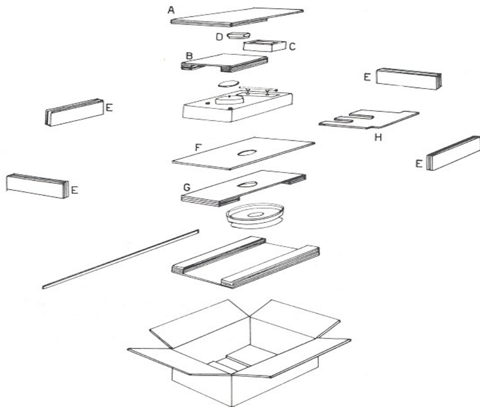
Fig. 2. Packing of the TD-150 AB and TD-150 B turntables.
