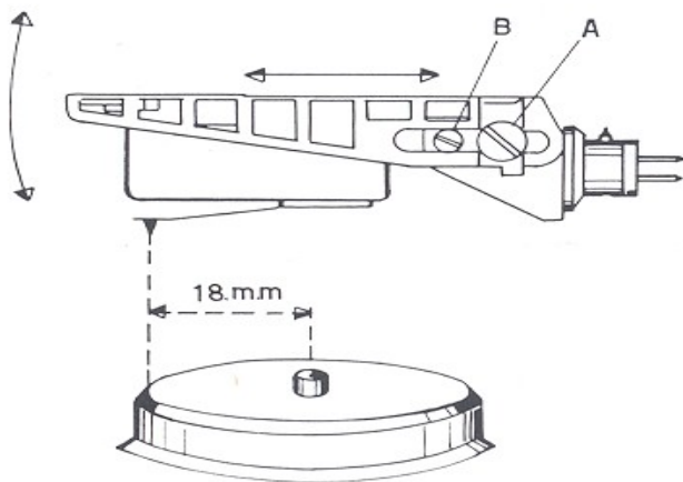
Fig. 7. Adjustment of plug-in shell.
