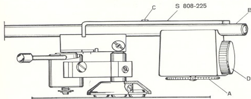
Fig. 8. Rear part of the pick-up arm.
